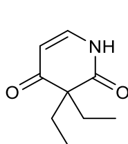
c) Pyrithyldion
