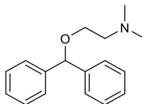
d) Diphenhydramin
